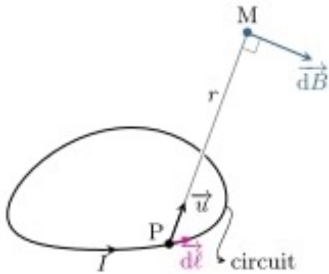
Illustration of the Biot-Savart formula.
